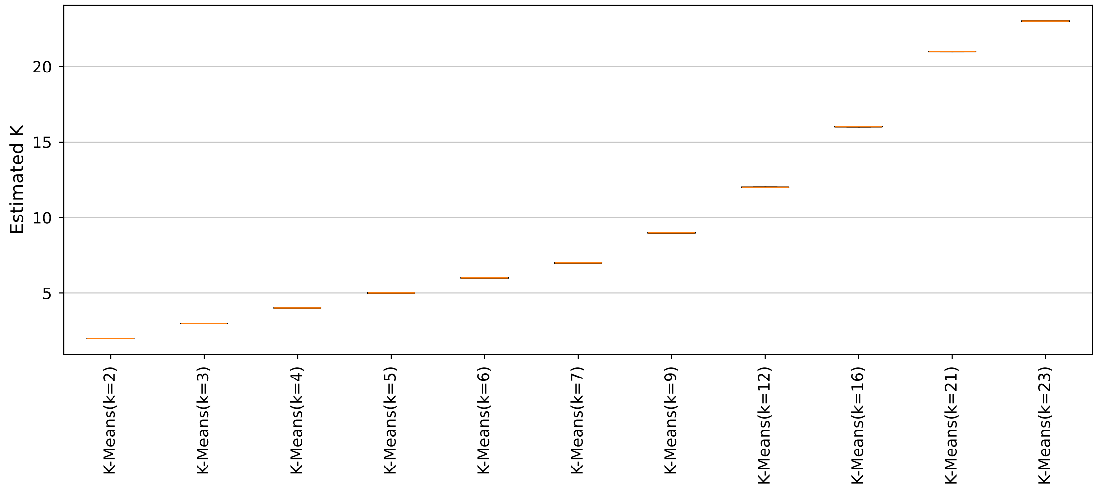
YARA Rules Estimated K Distribution (Cluster6_Size23 dataset)
